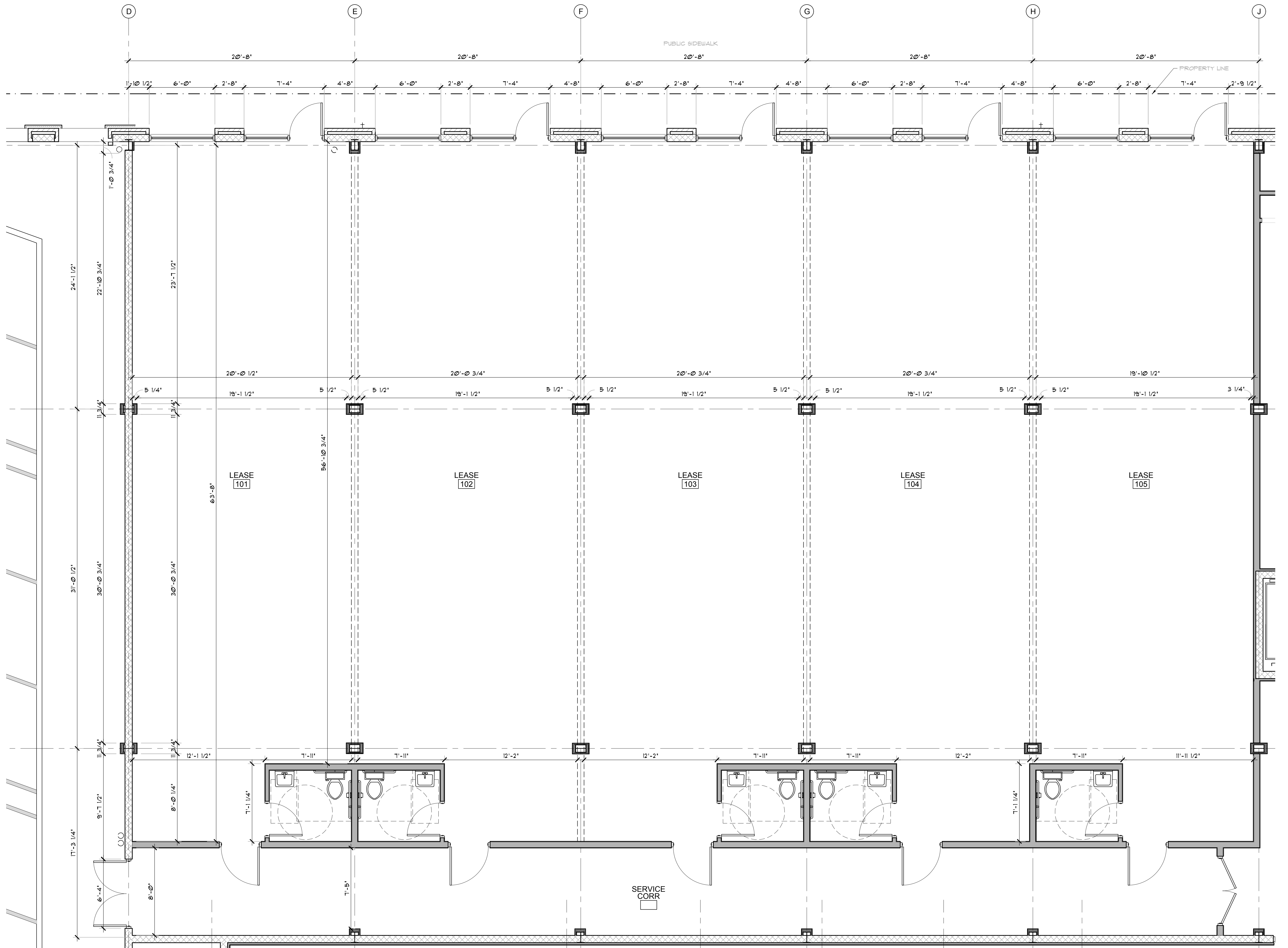
LEASE FLOOR PLAN SCALE: 1/4"=1'-0"
